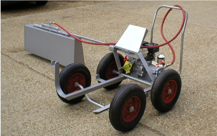
Spraybar shown in working position and shown being put in position on a Belspray Classic frame
